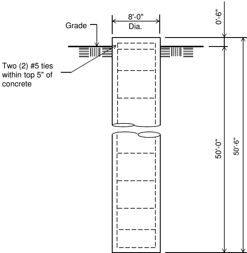
ELEVATION VIEW (94.02 Cu. Yds. each) (1 REQUIRED; NOT TO SCALE)
