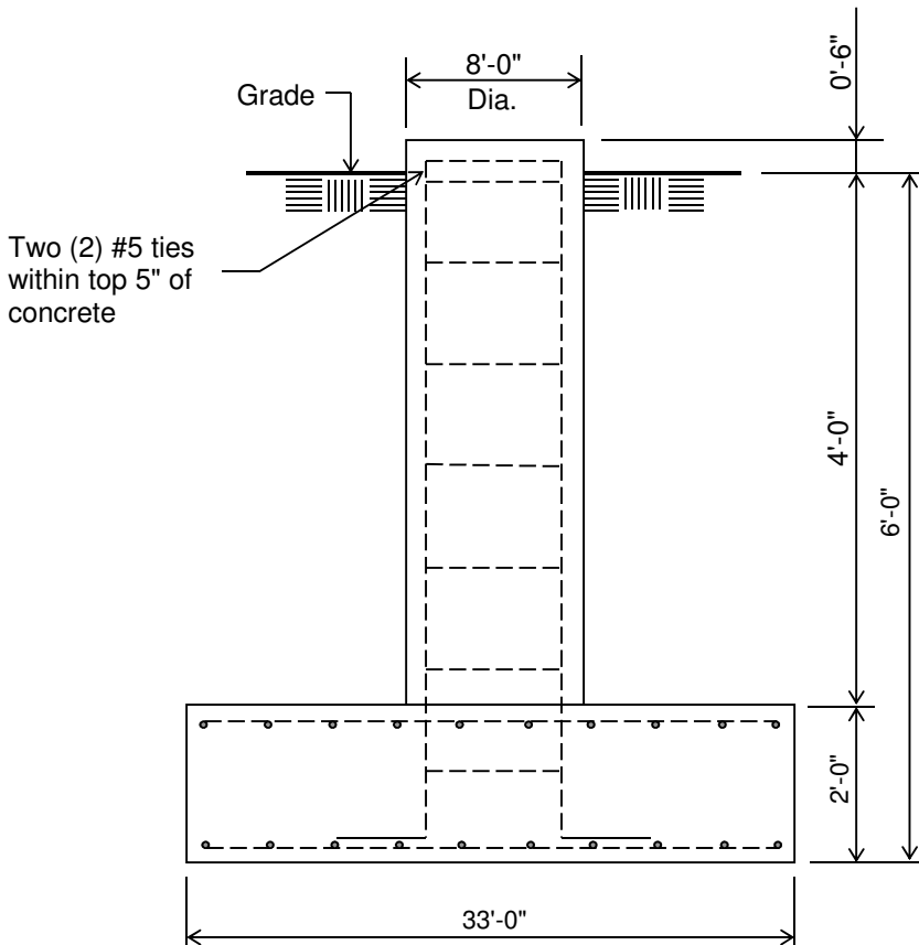
ELEVATION VIEW (89.04 Cu. Yds.) (1 REQUIRED; NOT TO SCALE)
